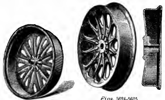
Fig. 5623. Inside View. Figs. 5624-5625. Outside View. Section. THE SHEFFIELD ALL-STEEL WHEEL. Drop Forged Hub; Wheel is made from one sheet of Steel.
